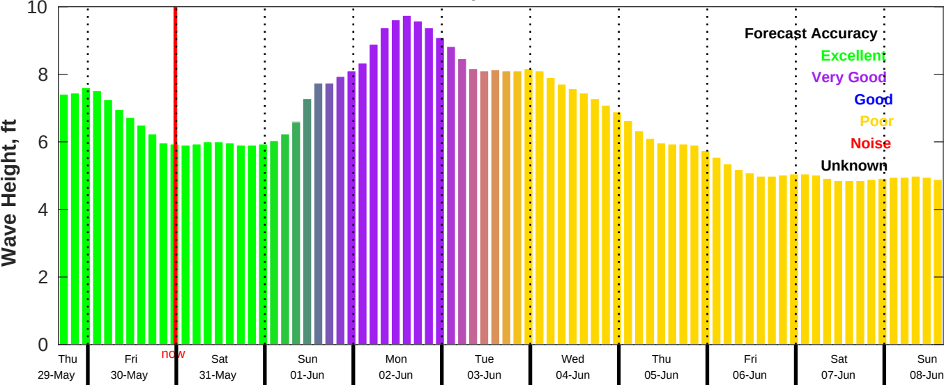
CMEMS Wave Forecast for NDBC 46011 from 29-May-2025 16:00:00 to 08-Jun-2025 16:00:00
