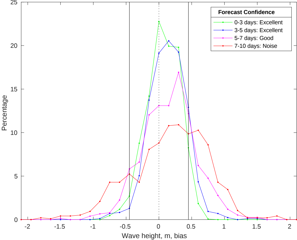
NDBC 46028 vs CMEMS Waves Bias Histogram: 31-May-2025
