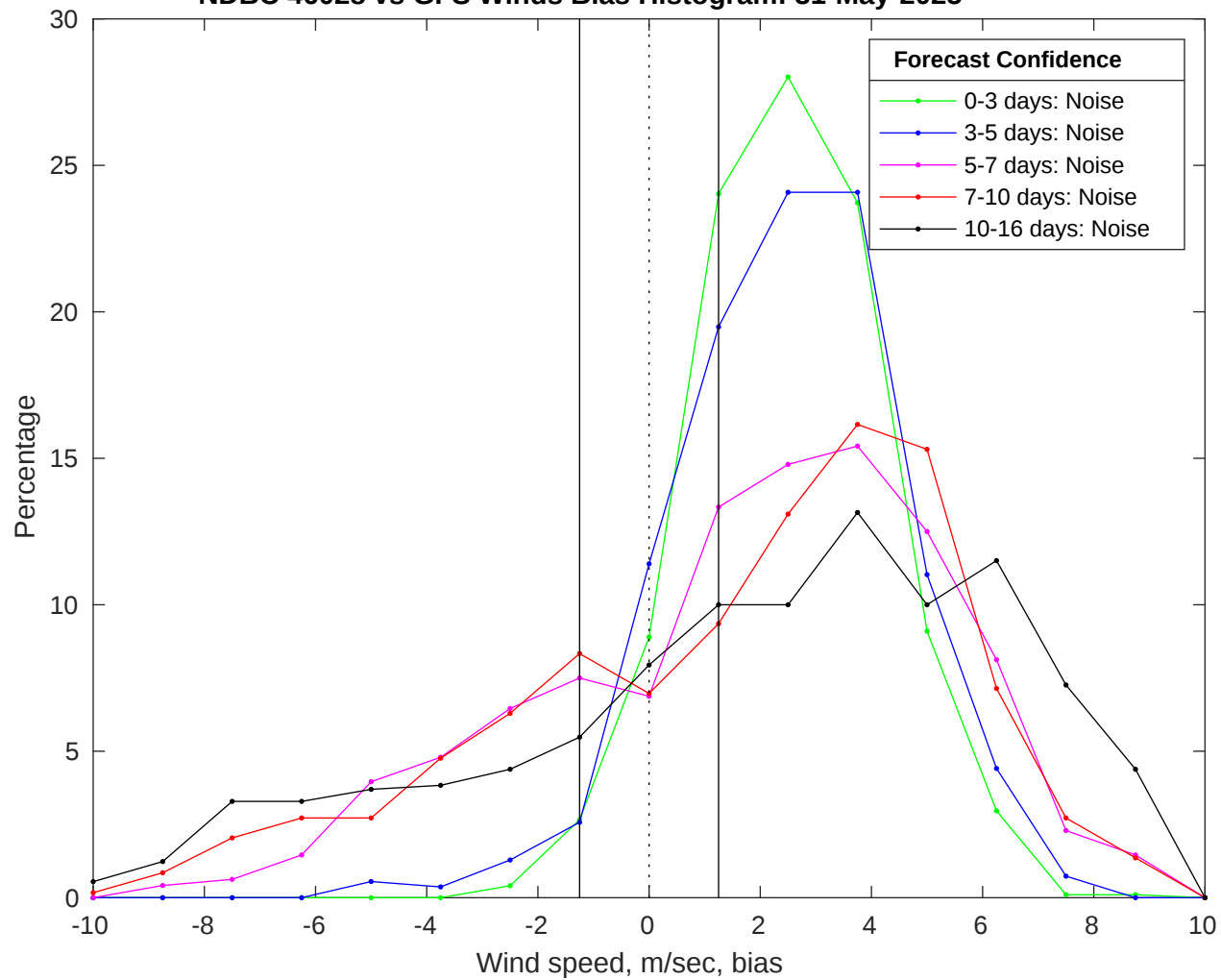
NDBC 46028 vs GFS Winds Bias Histogram: 31-May-2025
