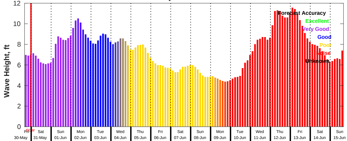
GFS Wave Forecast for NDBC 46028 from 30-May-2025 16:00:00 to 15-Jun-2025 16:00:00
