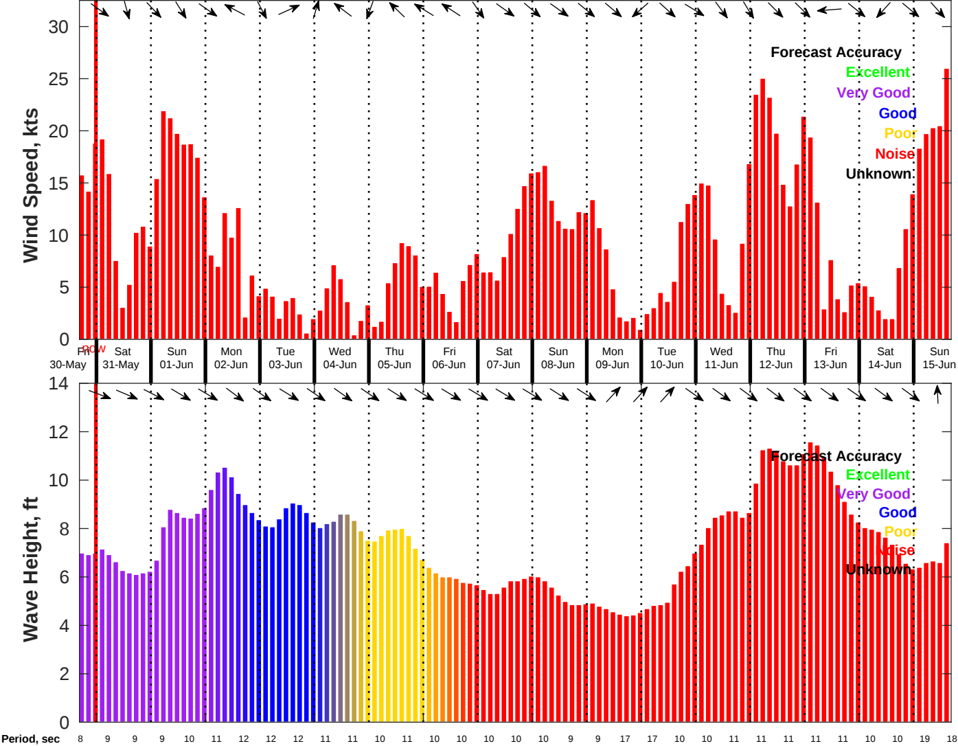
Wind & Wave Forecast for NDBC 46028 from 30-May-2025 16:00:00 to 15-Jun-2025 16:00:00
