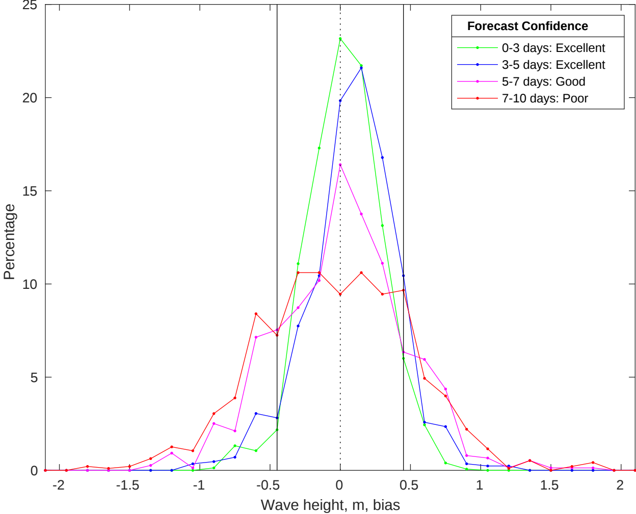
NDBC 46054 vs CMEMS Waves Bias Histogram: 31-May-2025
