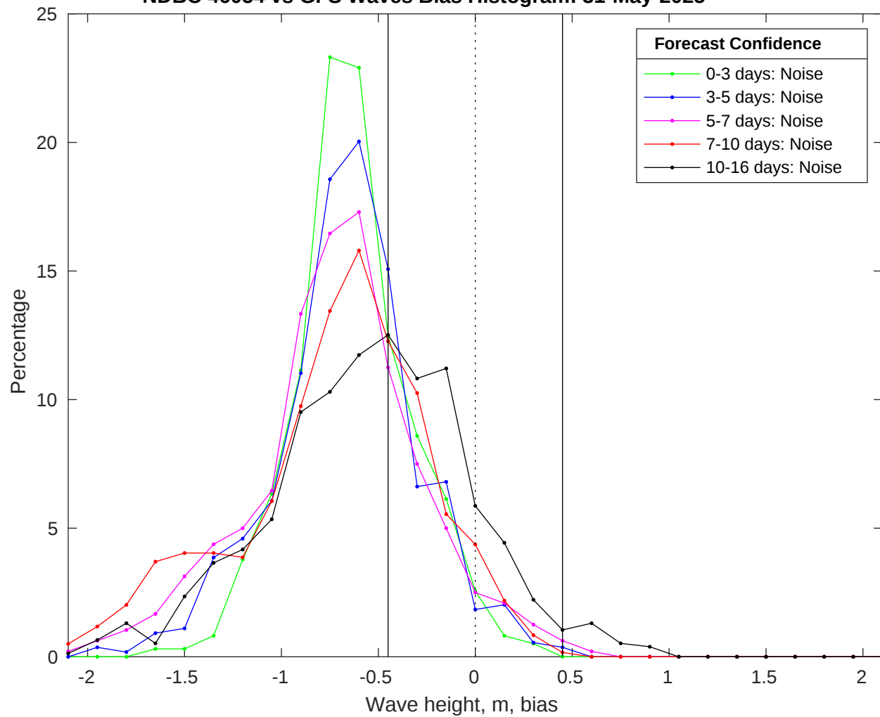
NDBC 46054 vs GFS Waves Bias Histogram: 31-May-2025
