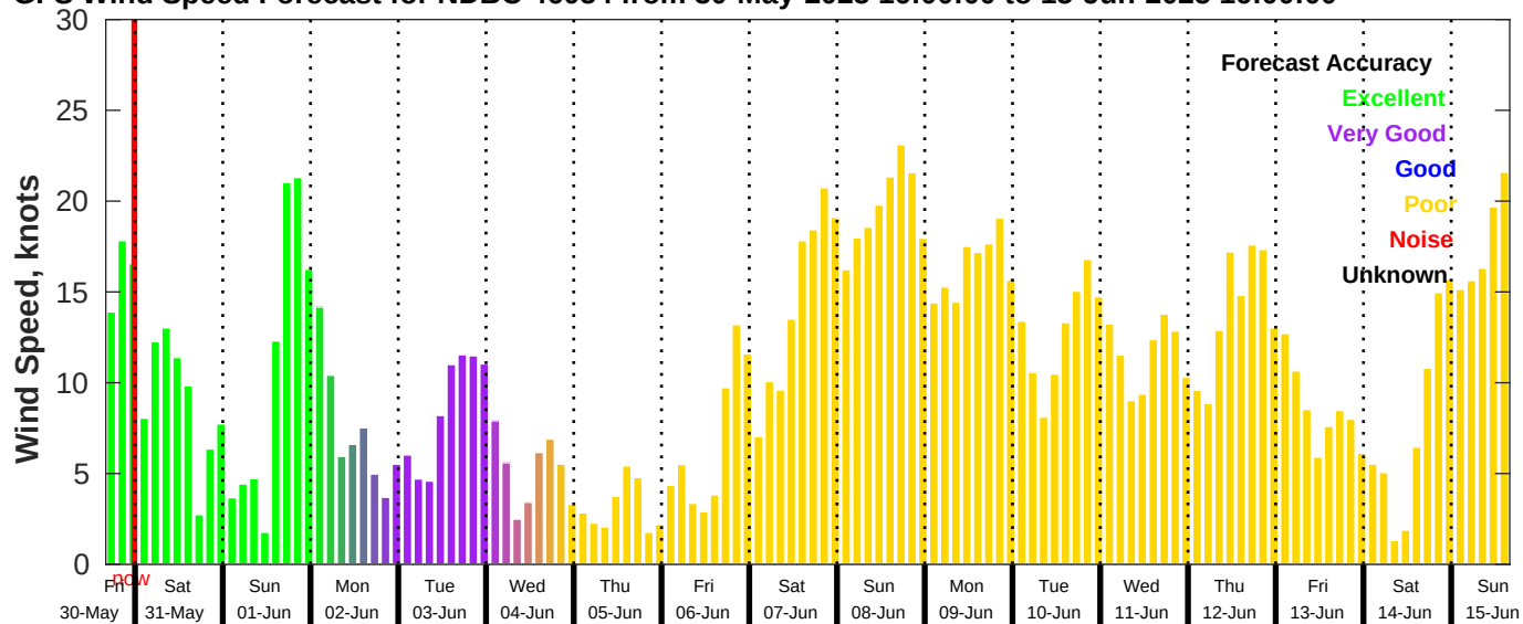
GFS Wind Speed Forecast for NDBC 46054 from 30-May-2025 16:00:00 to 15-Jun-2025 16:00:00
