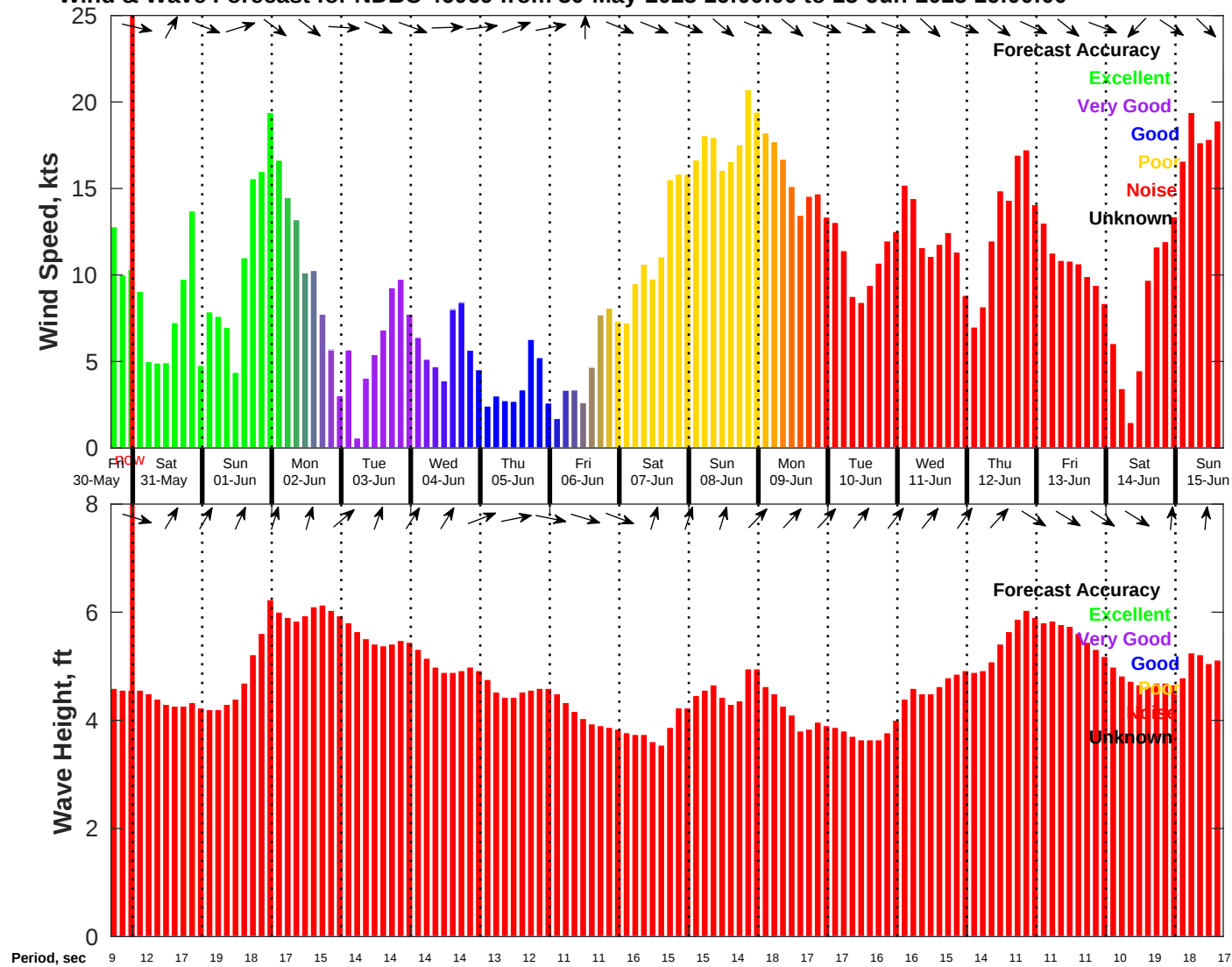
Wind & Wave Forecast for NDBC 46069 from 30-May-2025 16:00:00 to 15-Jun-2025 16:00:00
