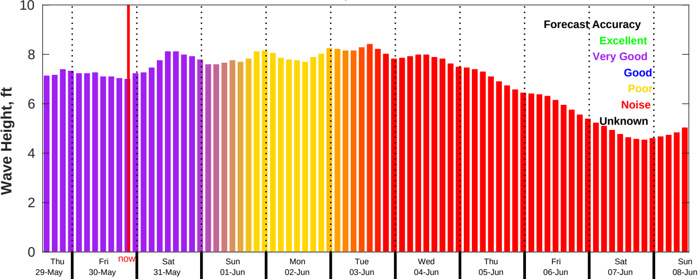
CMEMS Wave Forecast for NDBC 51209 from 29-May-2025 13:00:00 to 08-Jun-2025 13:00:00
