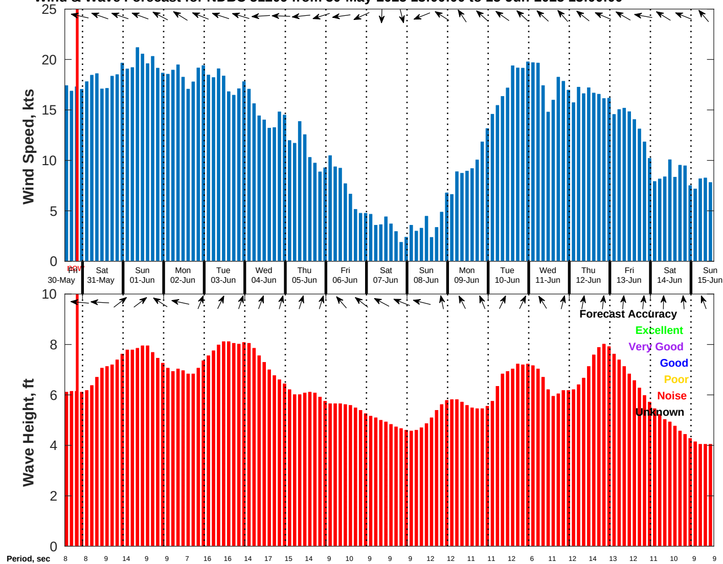
Wind & Wave Forecast for NDBC 51209 from 30-May-2025 13:00:00 to 15-Jun-2025 13:00:00
