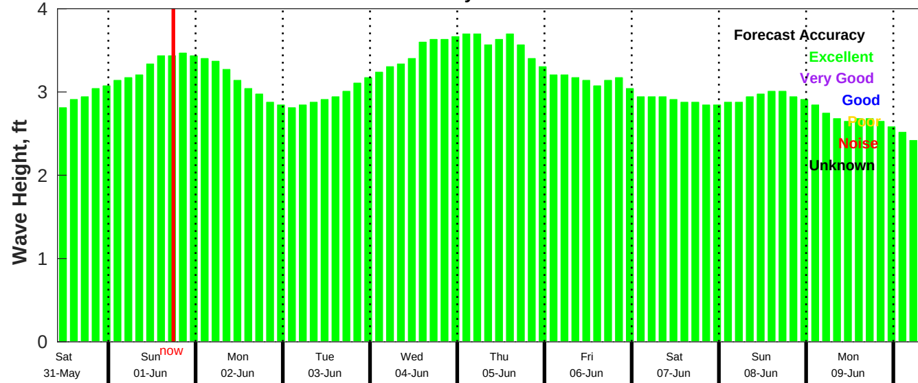
CMEMS Wave Forecast for NDBC 52211 from 30-May-2025 10:00:00 to 09-Jun-2025 10:00:00
