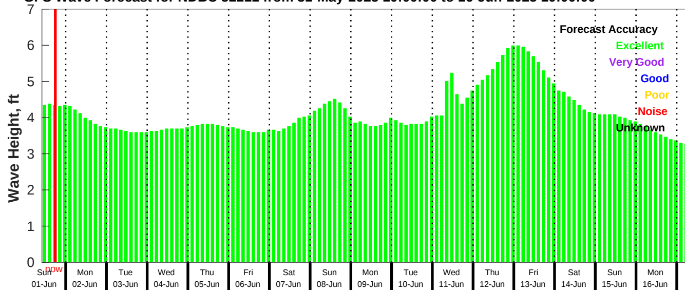
GFS Wave Forecast for NDBC 52211 from 31-May-2025 10:00:00 to 16-Jun-2025 10:00:00
