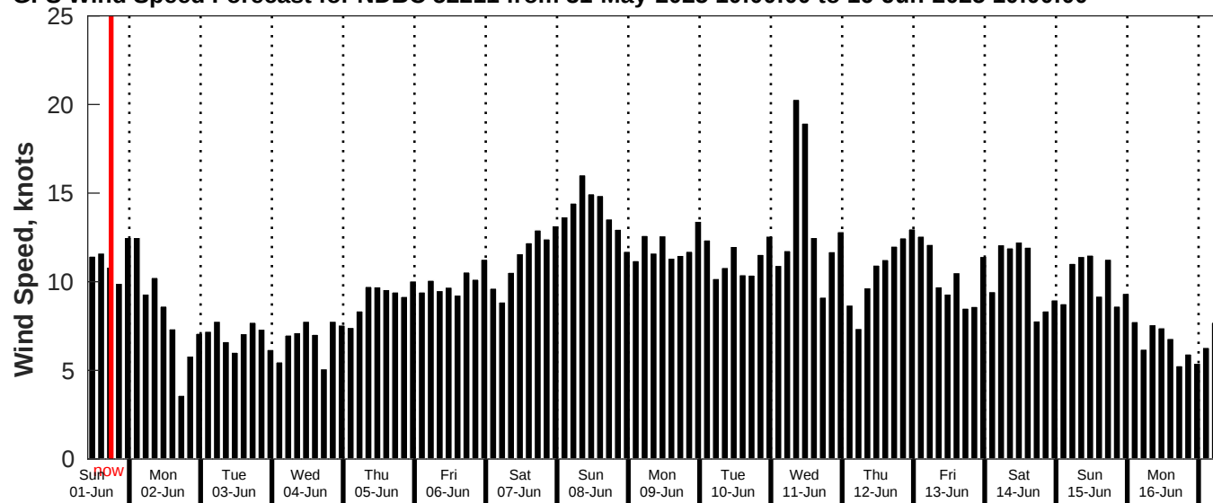
GFS Wind Speed Forecast for NDBC 52211 from 31-May-2025 10:00:00 to 16-Jun-2025 10:00:00
