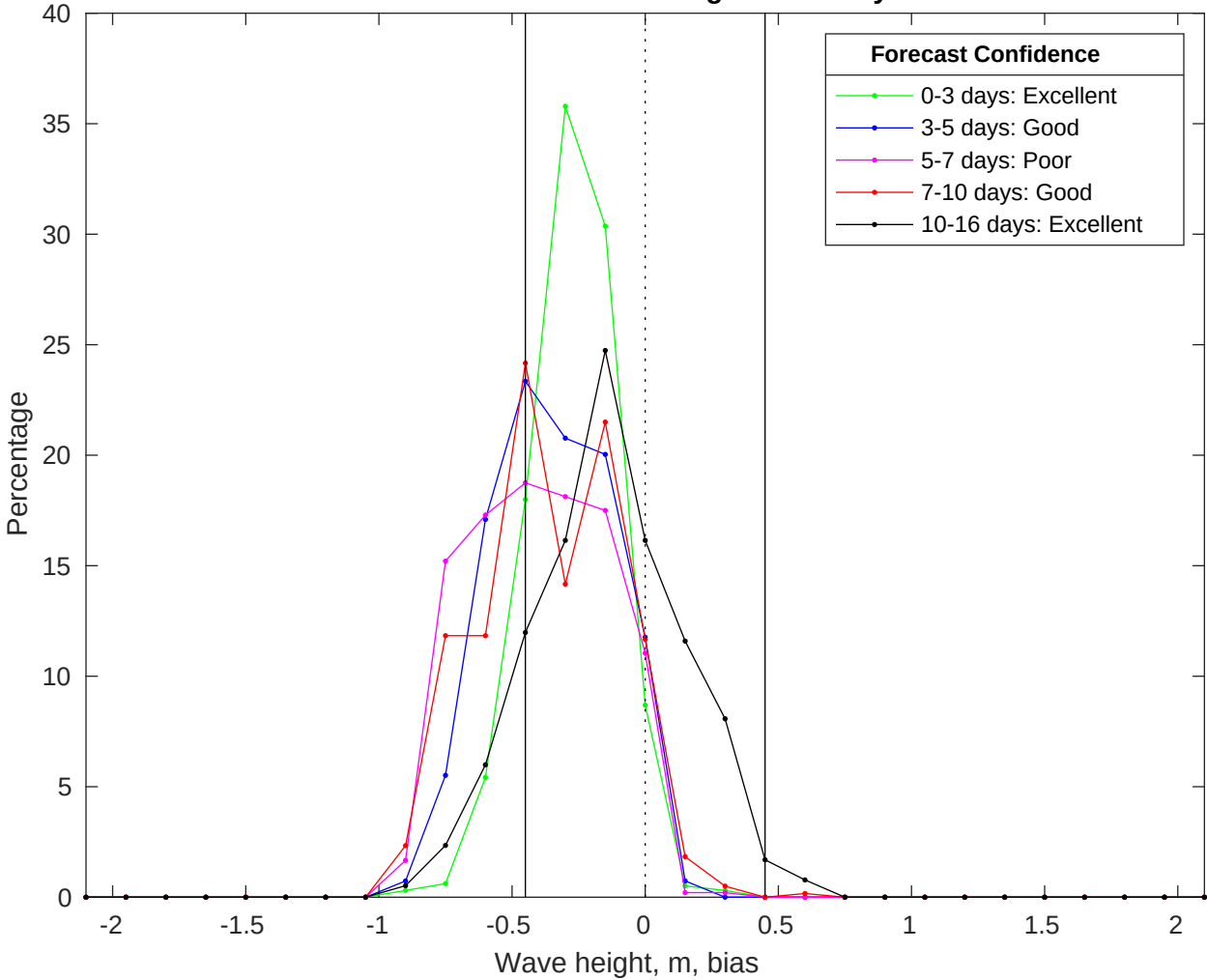
NDBC 52212 vs GFS Waves Bias Histogram: 31-May-2025
