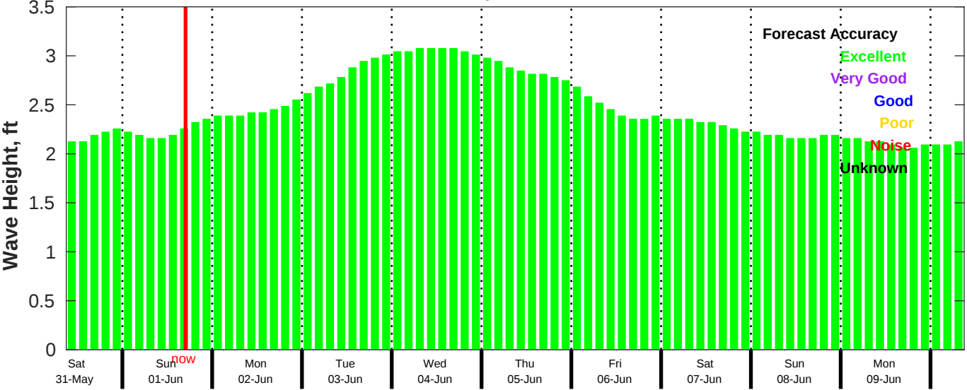
CMEMS Wave Forecast for NDBC 52212 from 30-May-2025 09:00:00 to 09-Jun-2025 09:00:00
