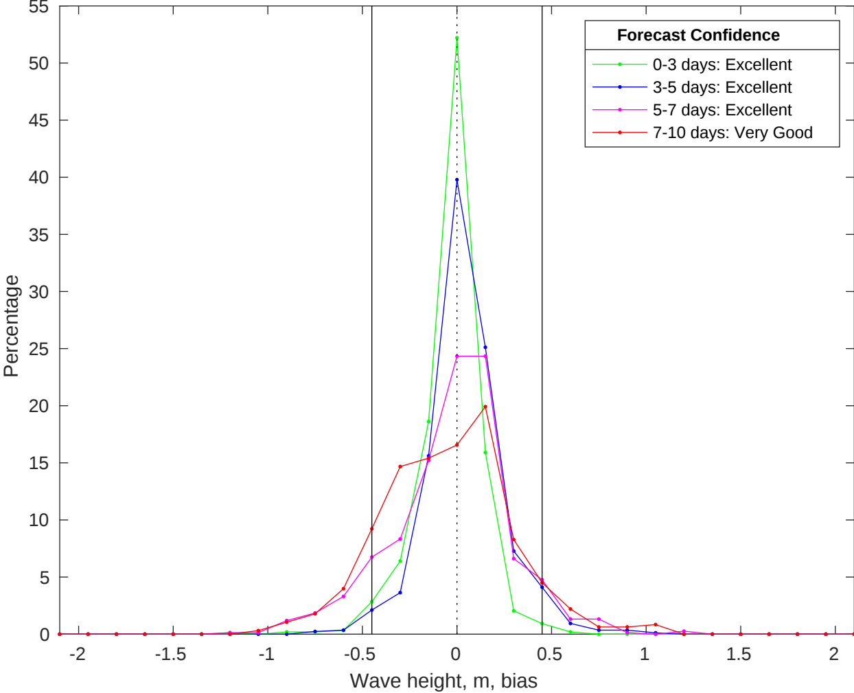
NDBC 41004 vs CMEMS Waves Bias Histogram: 01-Jun-2025
