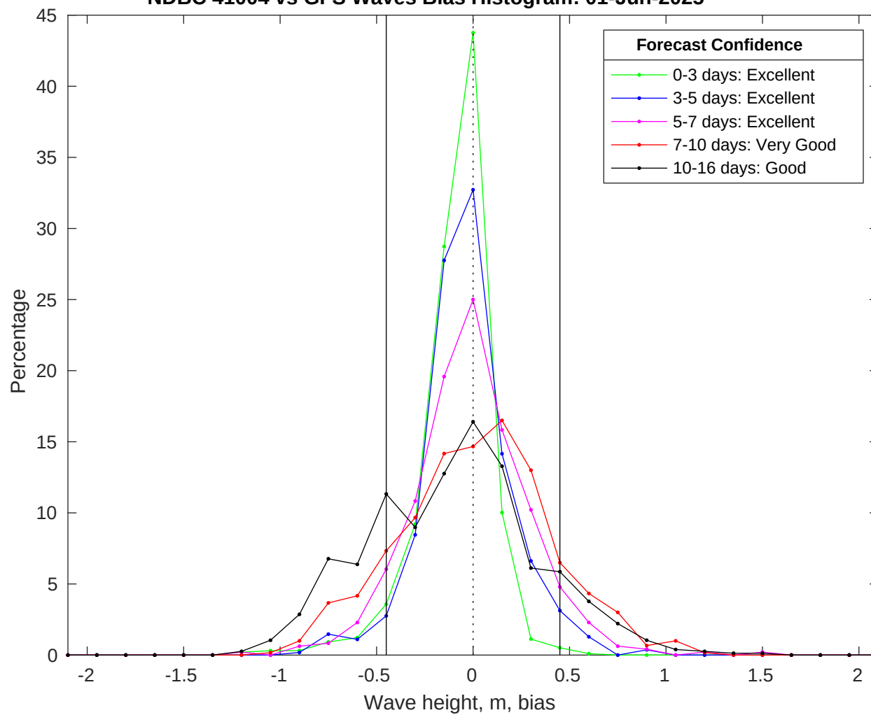
NDBC 41004 vs GFS Waves Bias Histogram: 01-Jun-2025
