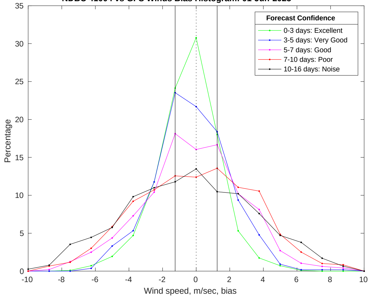
NDBC 41004 vs GFS Winds Bias Histogram: 01-Jun-2025
