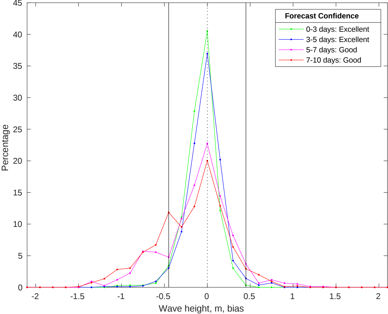
NDBC 41013 vs CMEMS Waves Bias Histogram: 01-Jun-2025
