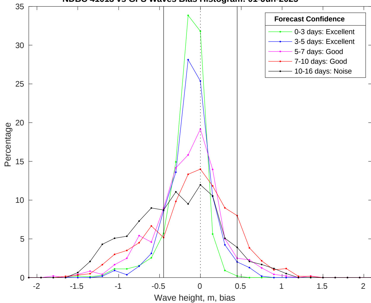
NDBC 41013 vs GFS Waves Bias Histogram: 01-Jun-2025
