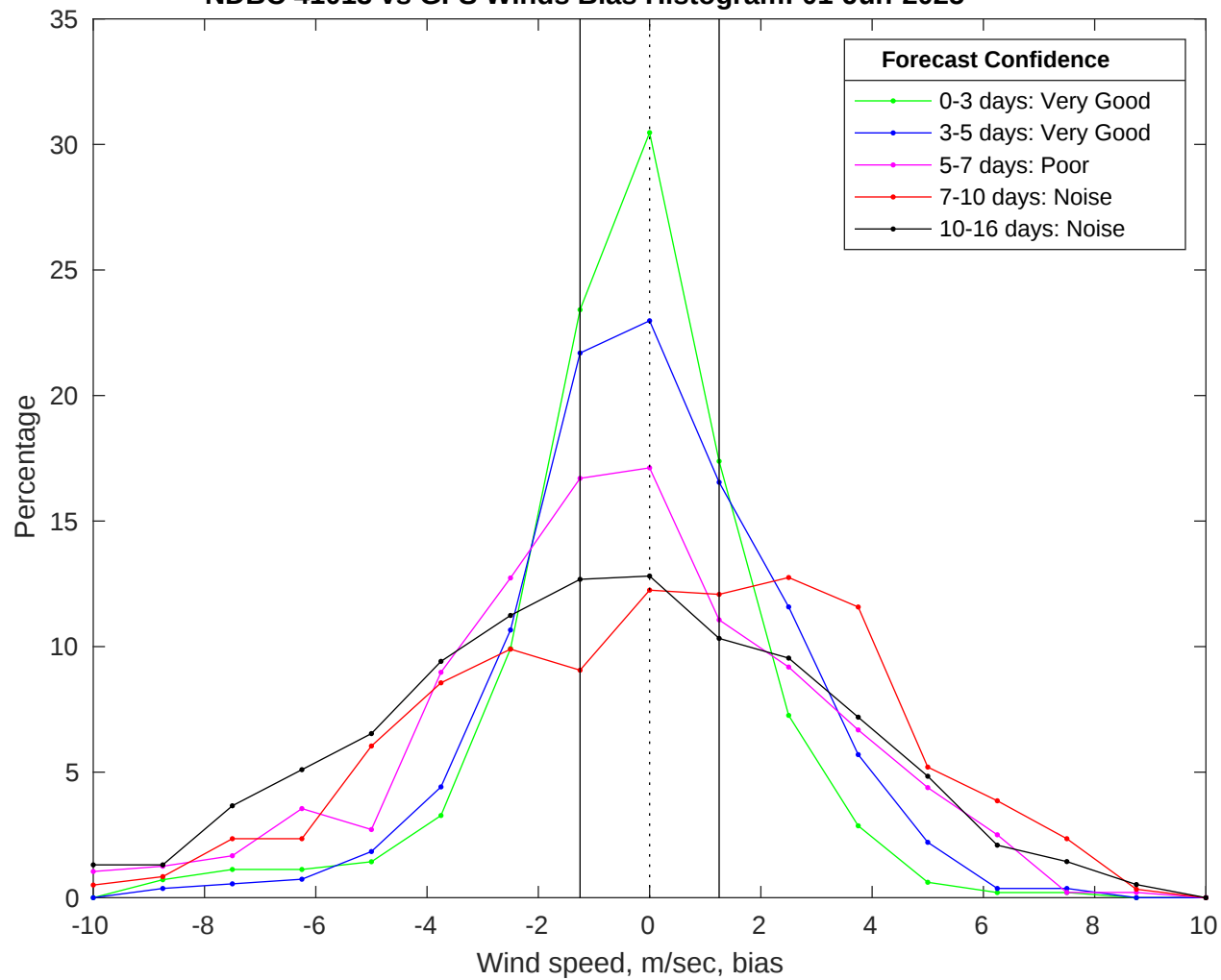
NDBC 41013 vs GFS Winds Bias Histogram: 01-Jun-2025
