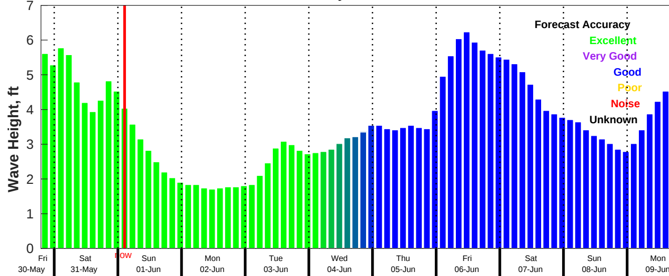
CMEMS Wave Forecast for NDBC 41013 from 30-May-2025 19:00:00 to 09-Jun-2025 19:00:00
