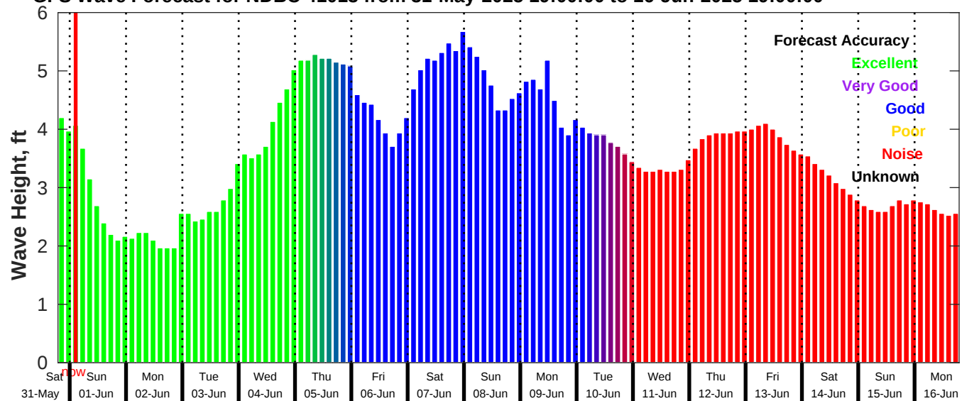
GFS Wave Forecast for NDBC 41013 from 31-May-2025 19:00:00 to 16-Jun-2025 19:00:00
