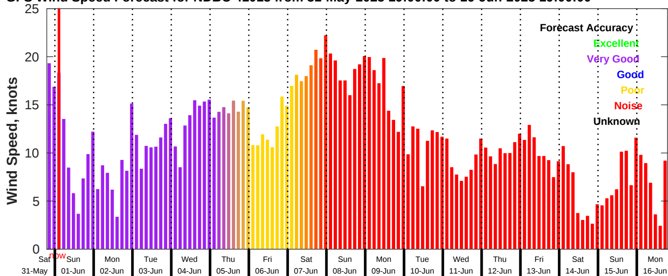
GFS Wind Speed Forecast for NDBC 41013 from 31-May-2025 19:00:00 to 16-Jun-2025 19:00:00
