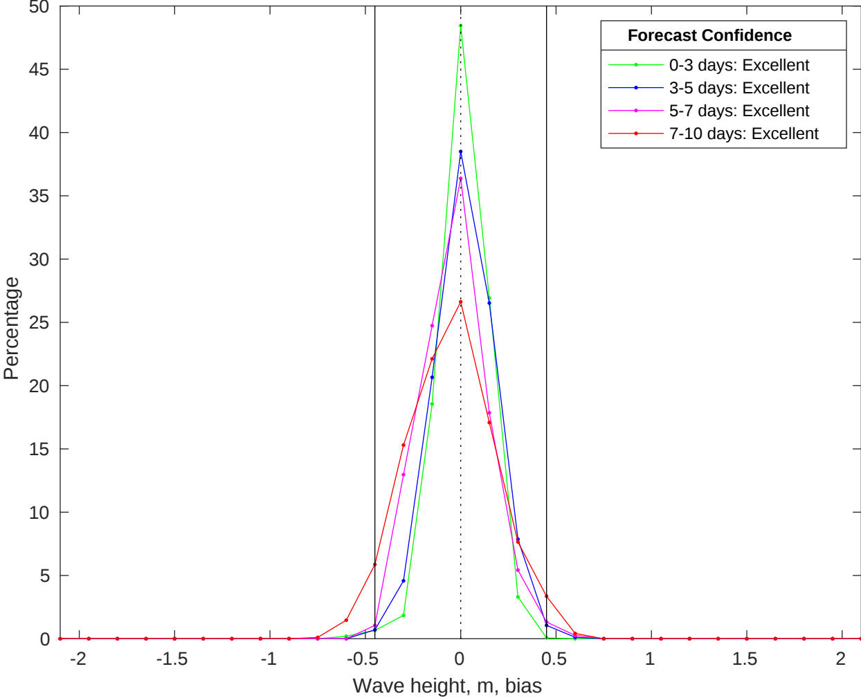
NDBC 41040 vs CMEMS Waves Bias Histogram: 01-Jun-2025
