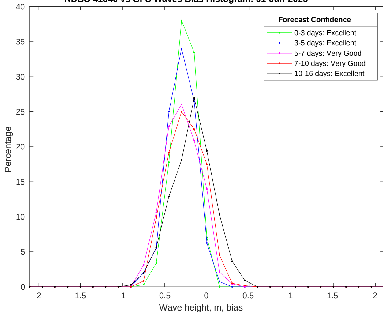
NDBC 41040 vs GFS Waves Bias Histogram: 01-Jun-2025
