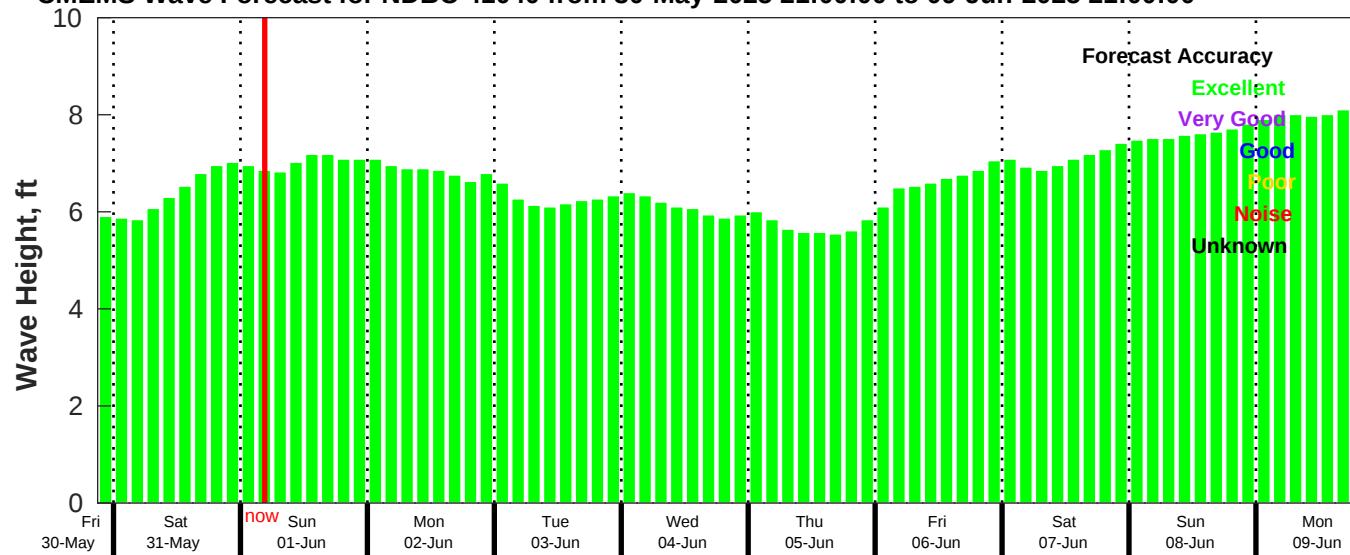
CMEMS Wave Forecast for NDBC 41040 from 30-May-2025 21:00:00 to 09-Jun-2025 21:00:00
