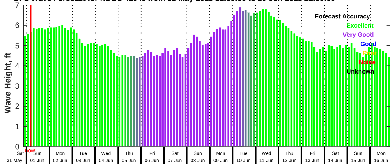
GFS Wave Forecast for NDBC 41040 from 31-May-2025 21:00:00 to 16-Jun-2025 21:00:00
