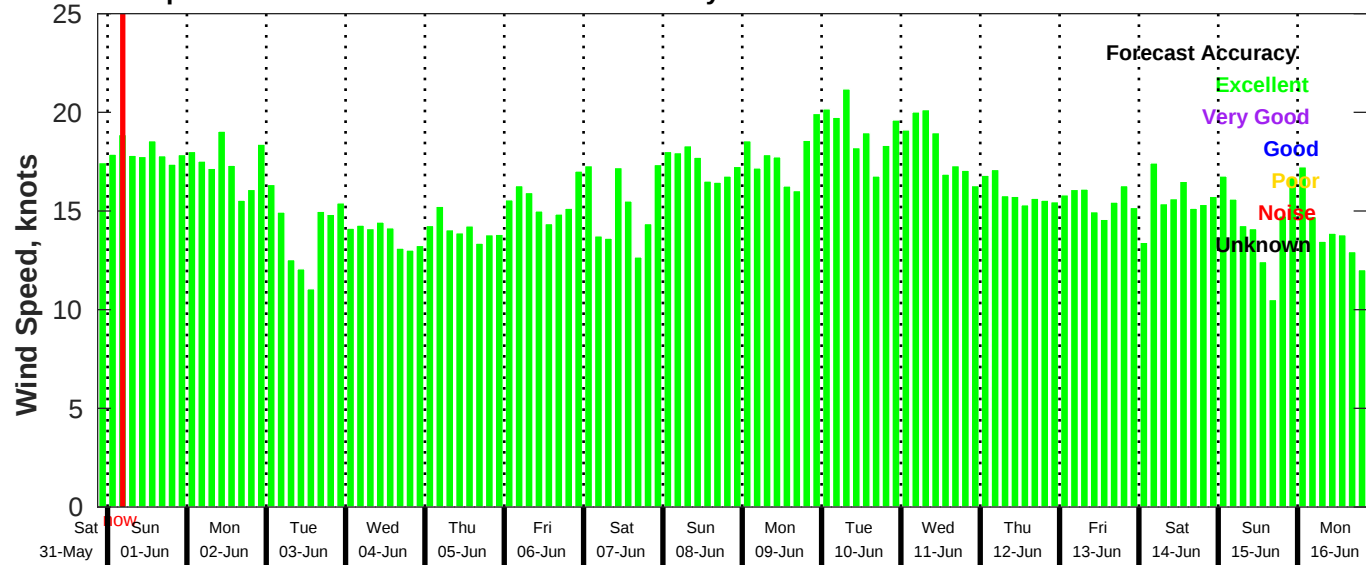
GFS Wind Speed Forecast for NDBC 41040 from 31-May-2025 21:00:00 to 16-Jun-2025 21:00:00
