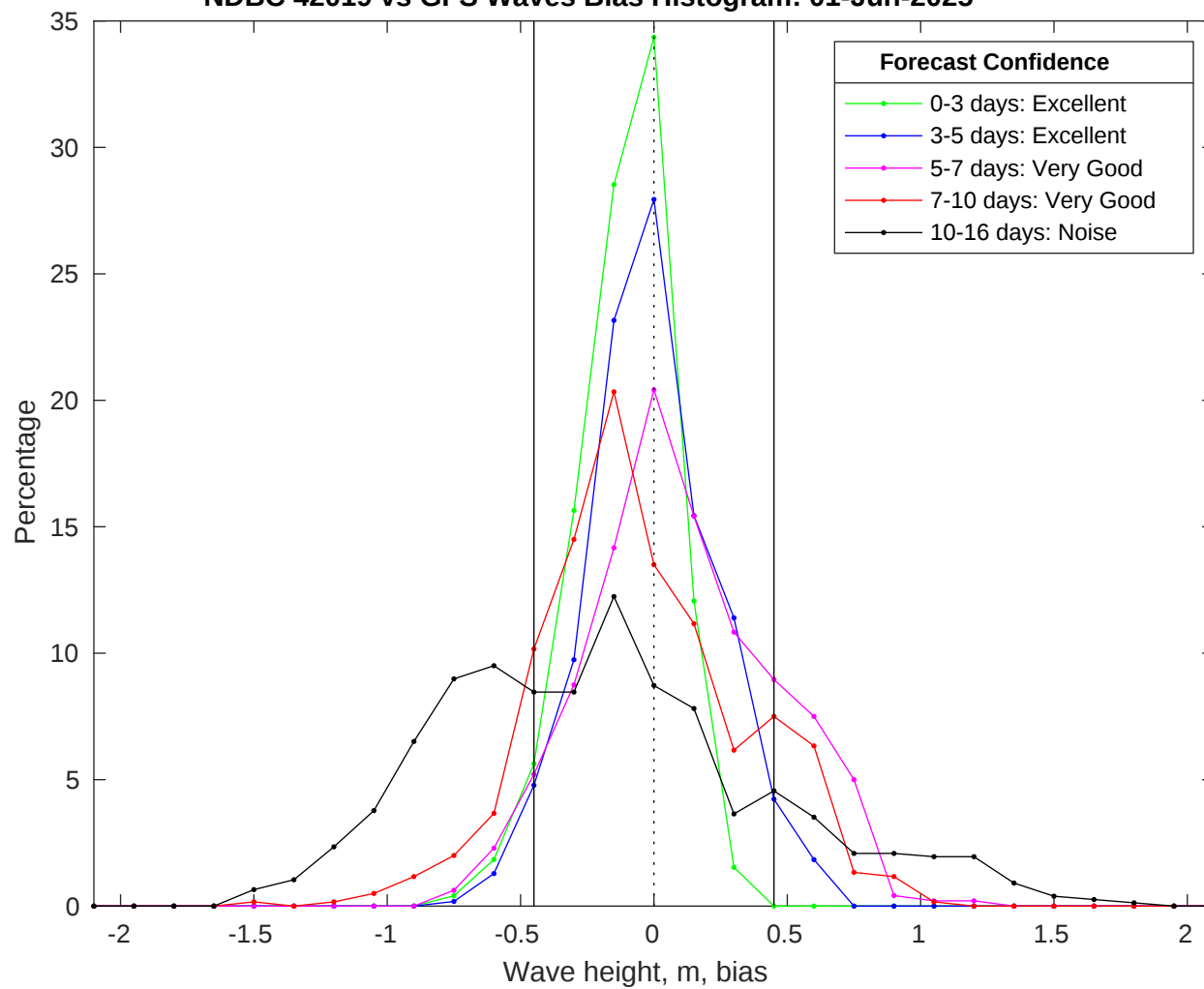
NDBC 42019 vs GFS Waves Bias Histogram: 01-Jun-2025
