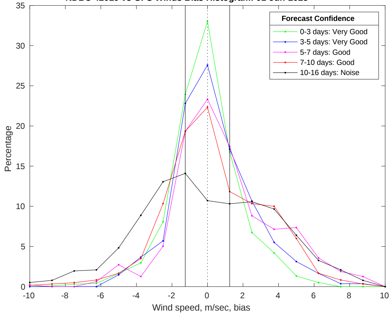
NDBC 42019 vs GFS Winds Bias Histogram: 01-Jun-2025
