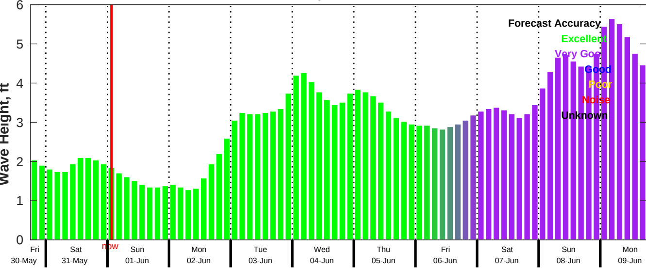
CMEMS Wave Forecast for NDBC 42019 from 30-May-2025 18:00:00 to 09-Jun-2025 18:00:00
