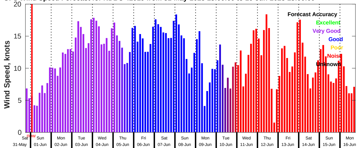
GFS Wind Speed Forecast for NDBC 42019 from 31-May-2025 18:00:00 to 16-Jun-2025 18:00:00
