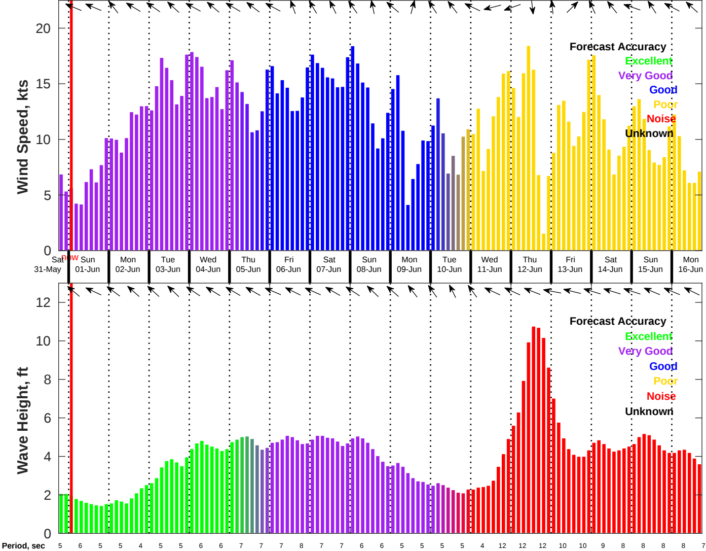
Wind & Wave Forecast for NDBC 42019 from 31-May-2025 18:00:00 to 16-Jun-2025 18:00:00
