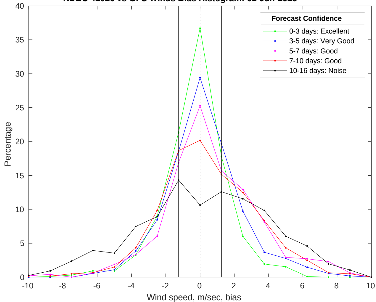
NDBC 42020 vs GFS Winds Bias Histogram: 01-Jun-2025
