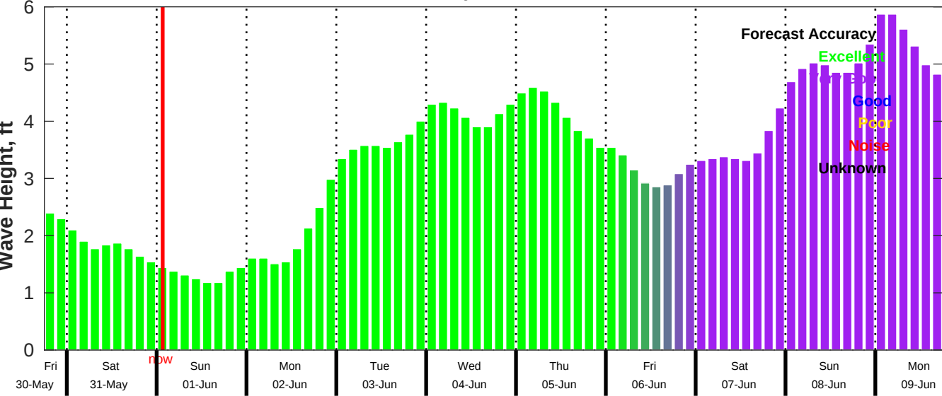
CMEMS Wave Forecast for NDBC 42020 from 30-May-2025 18:00:00 to 09-Jun-2025 18:00:00
