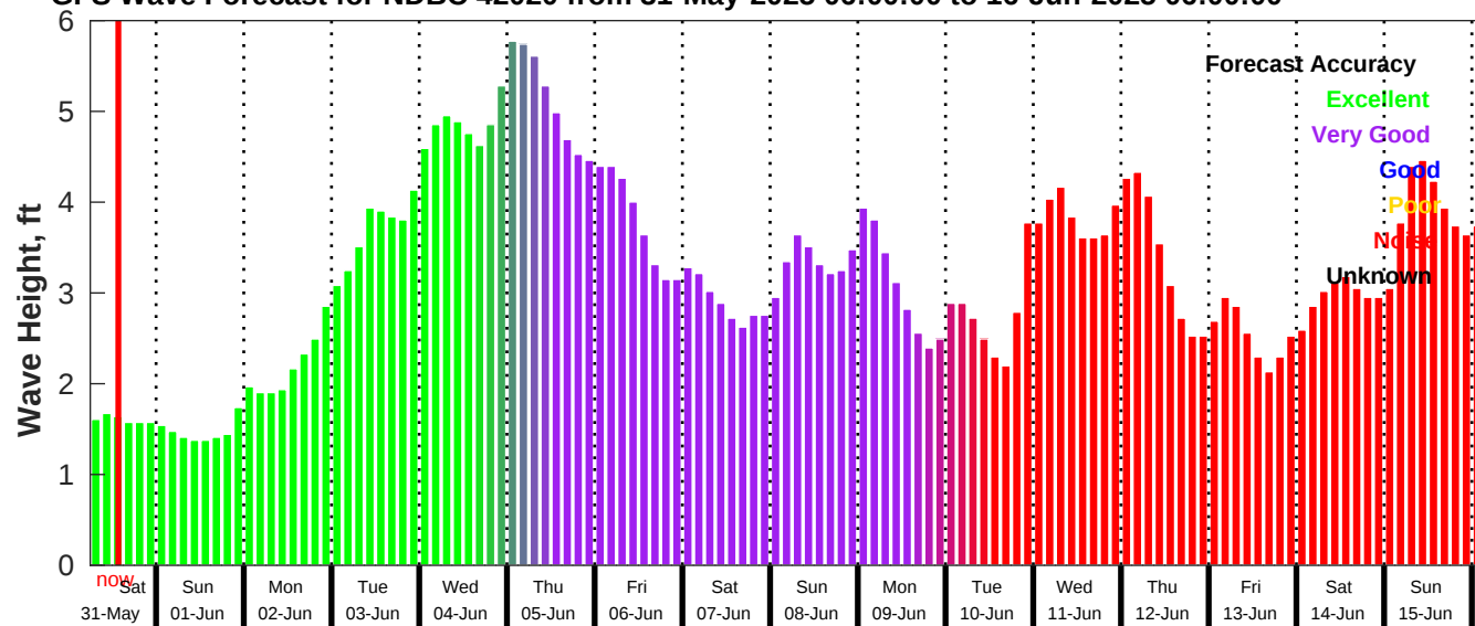
GFS Wave Forecast for NDBC 42020 from 31-May-2025 06:00:00 to 16-Jun-2025 06:00:00
