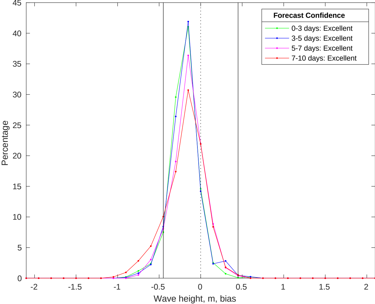
NDBC 42035 vs CMEMS Waves Bias Histogram: 01-Jun-2025
