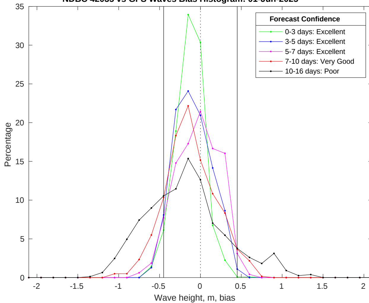
NDBC 42035 vs GFS Waves Bias Histogram: 01-Jun-2025
