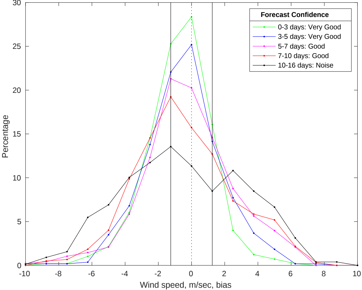
NDBC 42035 vs GFS Winds Bias Histogram: 01-Jun-2025
