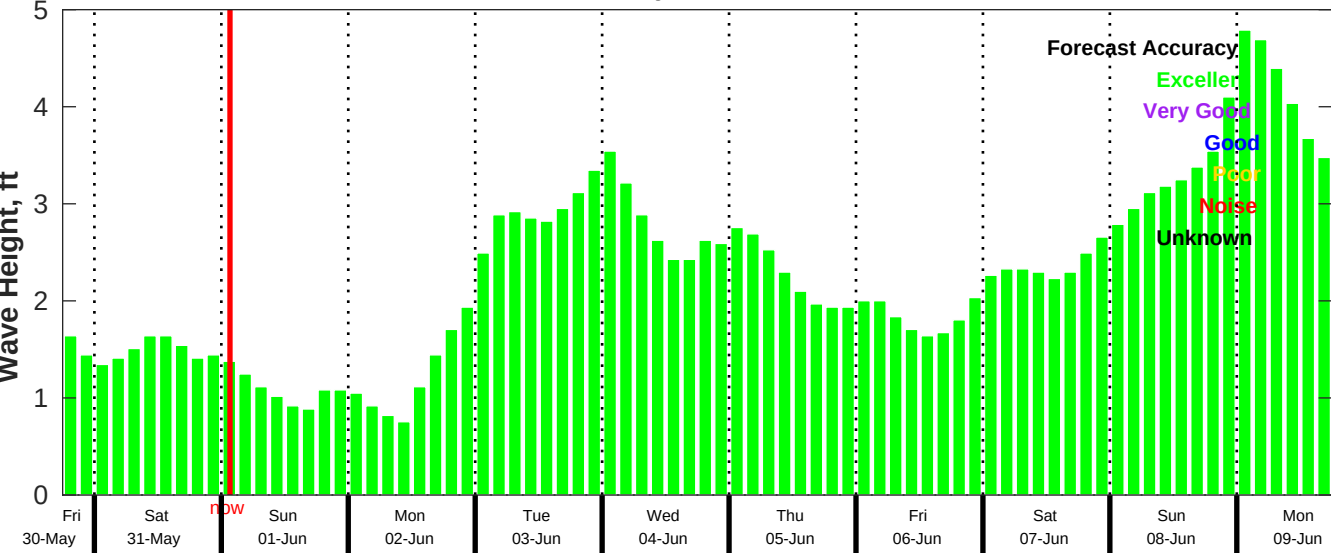
CMEMS Wave Forecast for NDBC 42035 from 30-May-2025 18:00:00 to 09-Jun-2025 18:00:00
