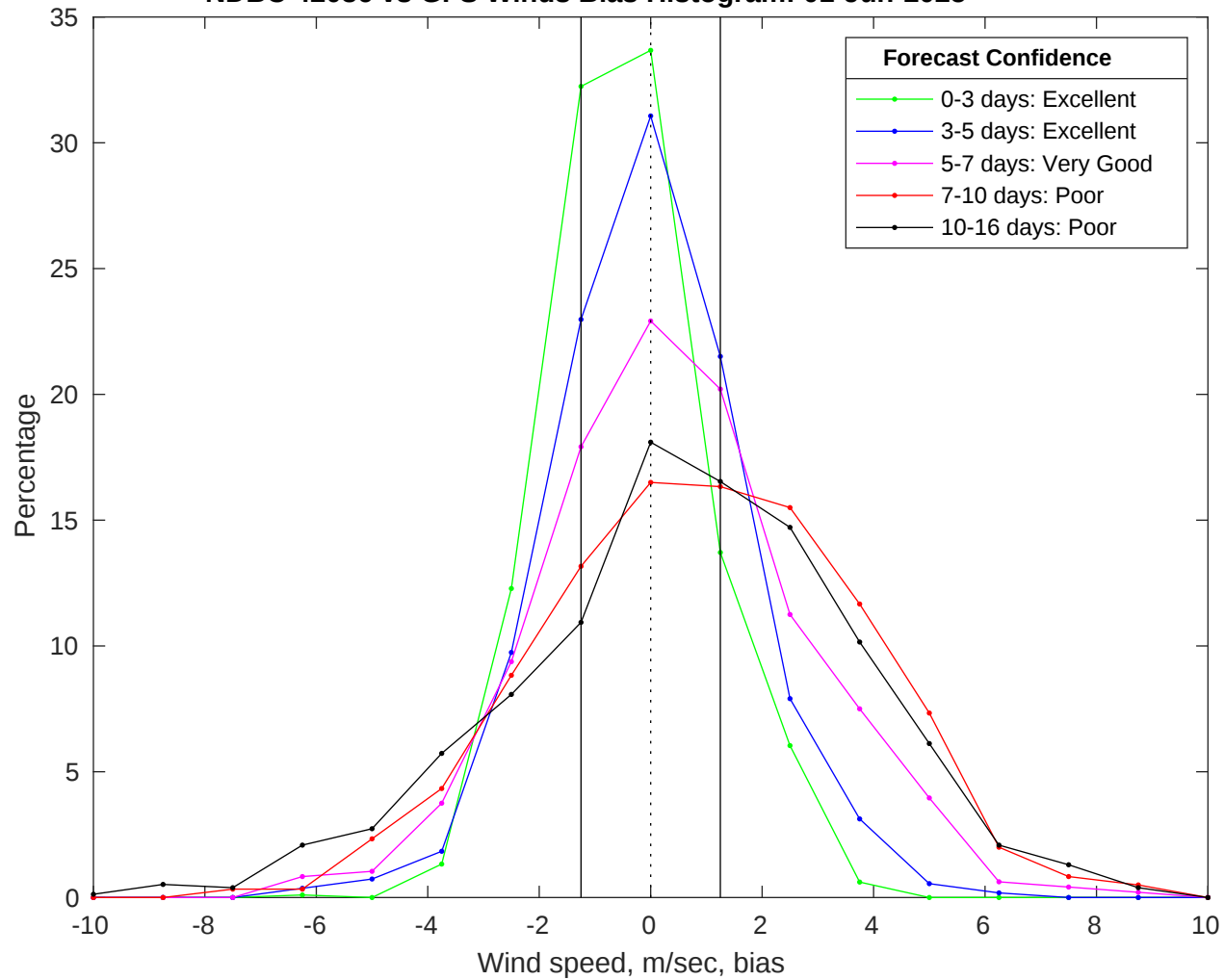
NDBC 42036 vs GFS Winds Bias Histogram: 01-Jun-2025
