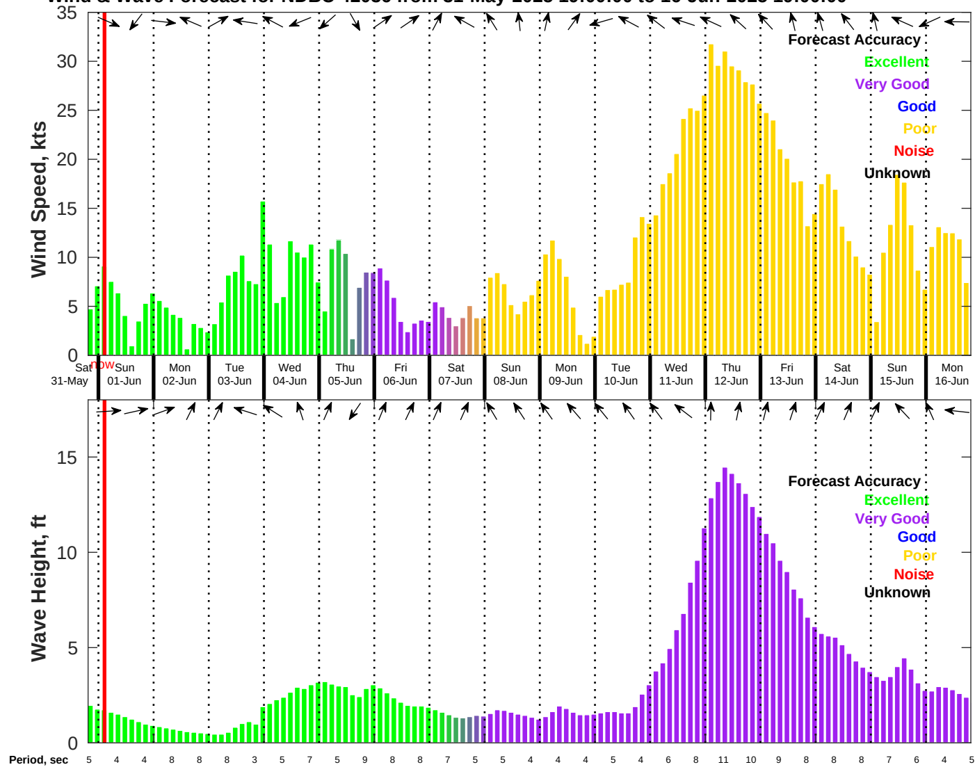
Wind & Wave Forecast for NDBC 42036 from 31-May-2025 19:00:00 to 16-Jun-2025 19:00:00
