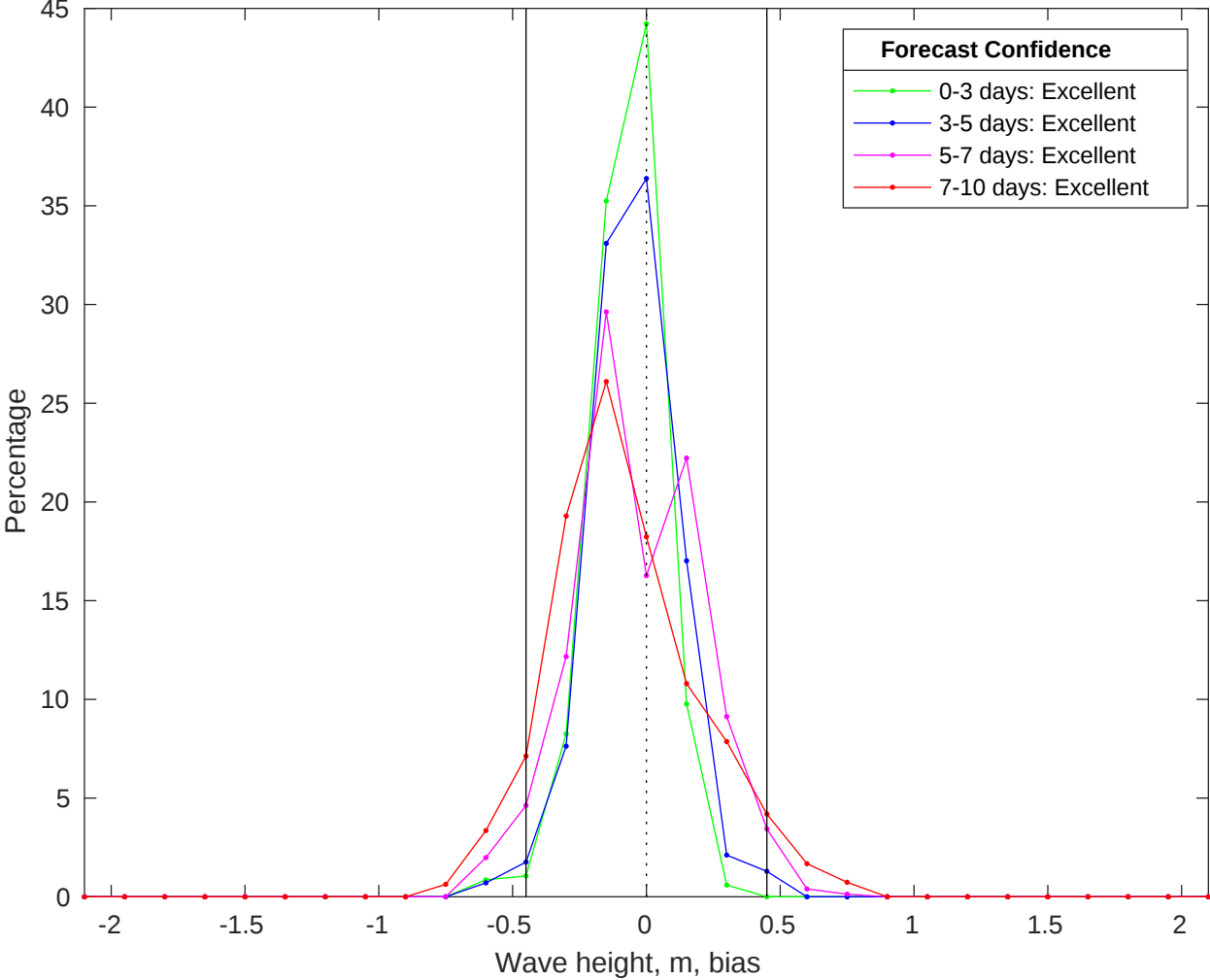
NDBC 42040 vs CMEMS Waves Bias Histogram: 01-Jun-2025
