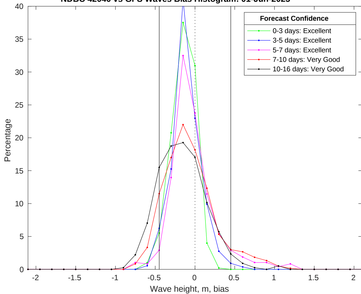
NDBC 42040 vs GFS Waves Bias Histogram: 01-Jun-2025
