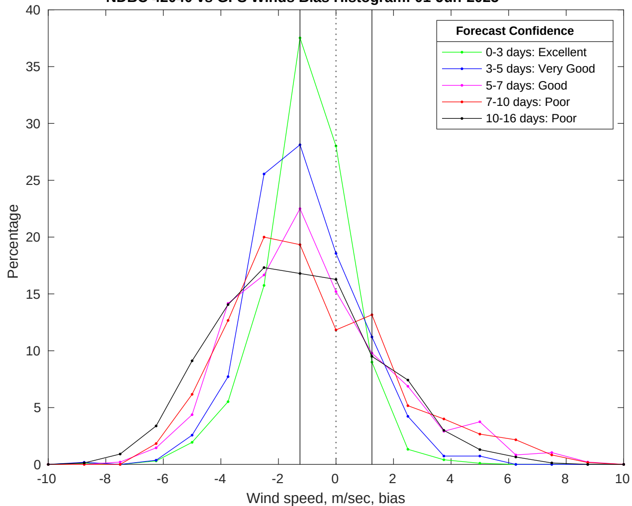
NDBC 42040 vs GFS Winds Bias Histogram: 01-Jun-2025
