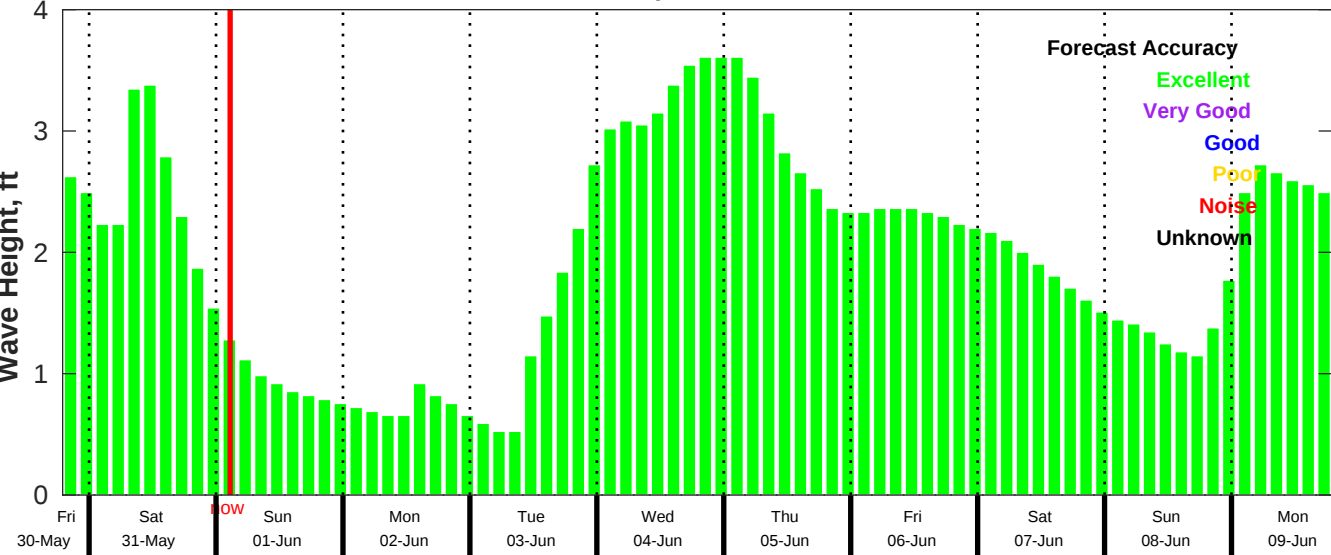
CMEMS Wave Forecast for NDBC 42040 from 30-May-2025 19:00:00 to 09-Jun-2025 19:00:00
