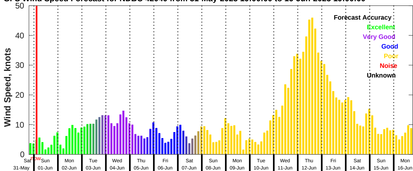
GFS Wind Speed Forecast for NDBC 42040 from 31-May-2025 19:00:00 to 16-Jun-2025 19:00:00
