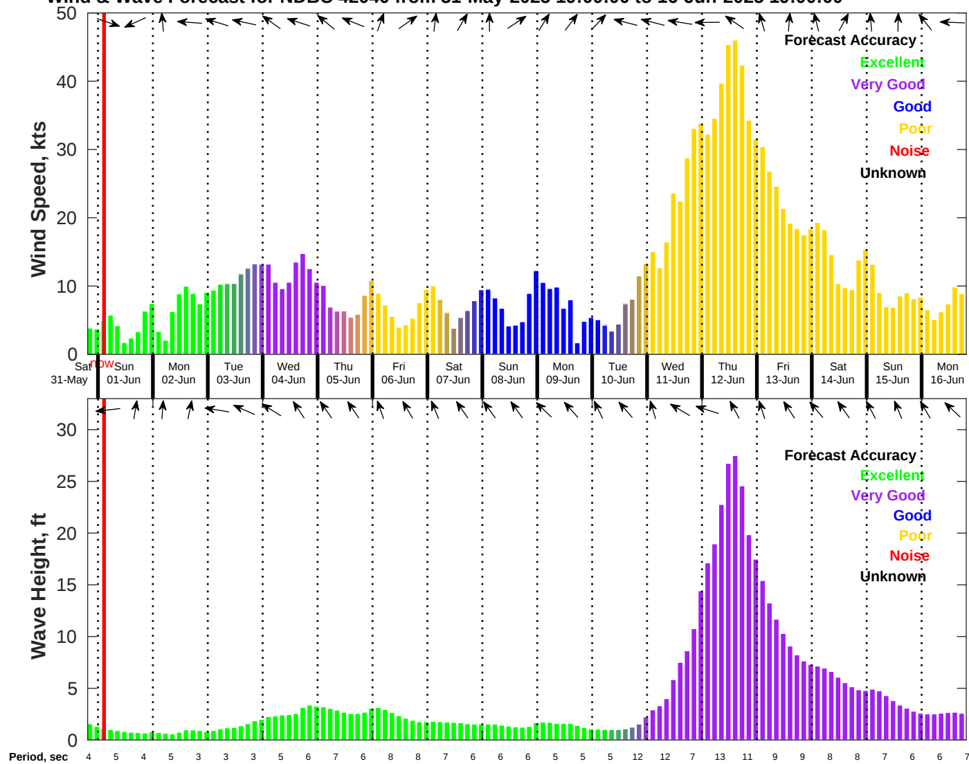
Wind & Wave Forecast for NDBC 42040 from 31-May-2025 19:00:00 to 16-Jun-2025 19:00:00
